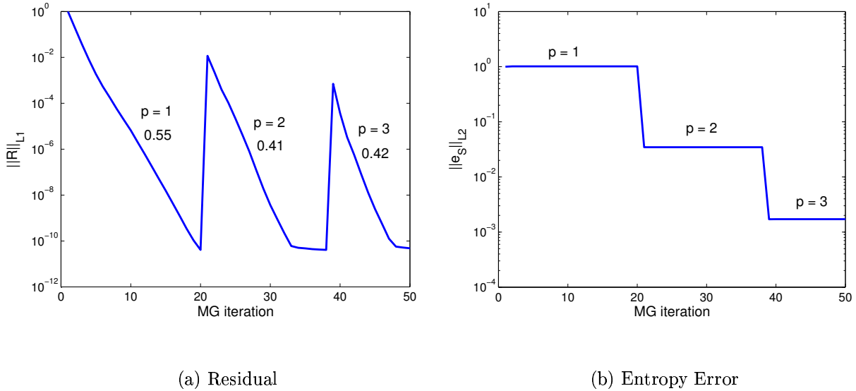
Figure 6: 2-D duct (1296 elements): FMG history with full convergence on each level.
