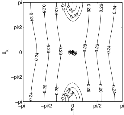
(c) AR = 1, Re = 10
