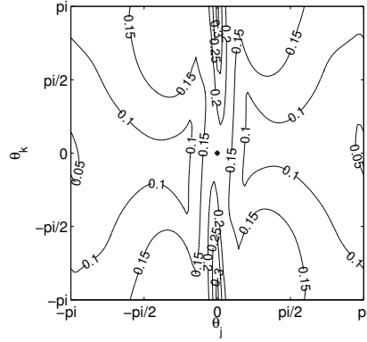
(b) AR = 1, Re = 100
