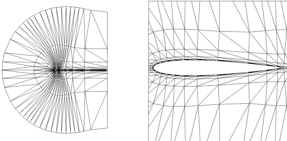
Figure 10: Coarse NACA 0012 mesh, 672 elements.
