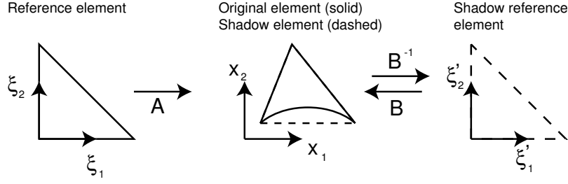
Figure 16: Reference and shadow triangles corresponding to a curved element.
