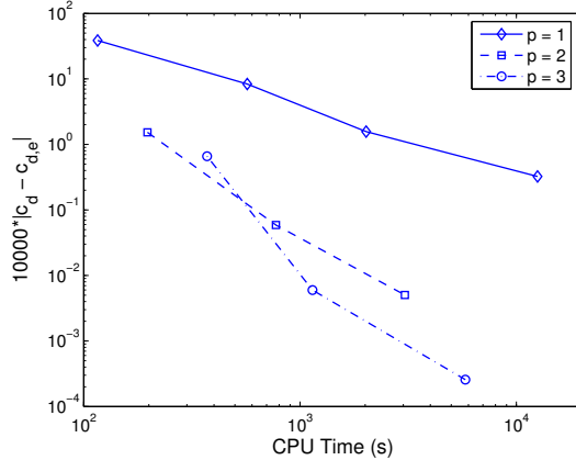
Figure 12: Drag error versus CPU time for NACA 0012 at M = 0.5 , Re = 5000 , \alpha = 0^\circ .
