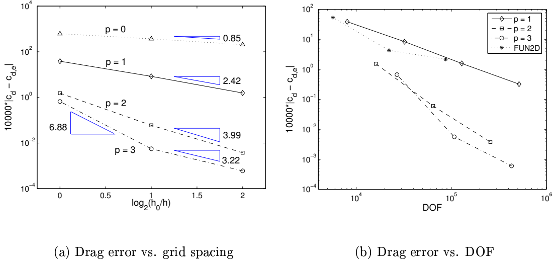
Figure 11: Drag error results for 0 \leq p \leq 3 for NACA 0012 at M = 0.5 , Re = 5000 , \alpha = 0^\circ .
