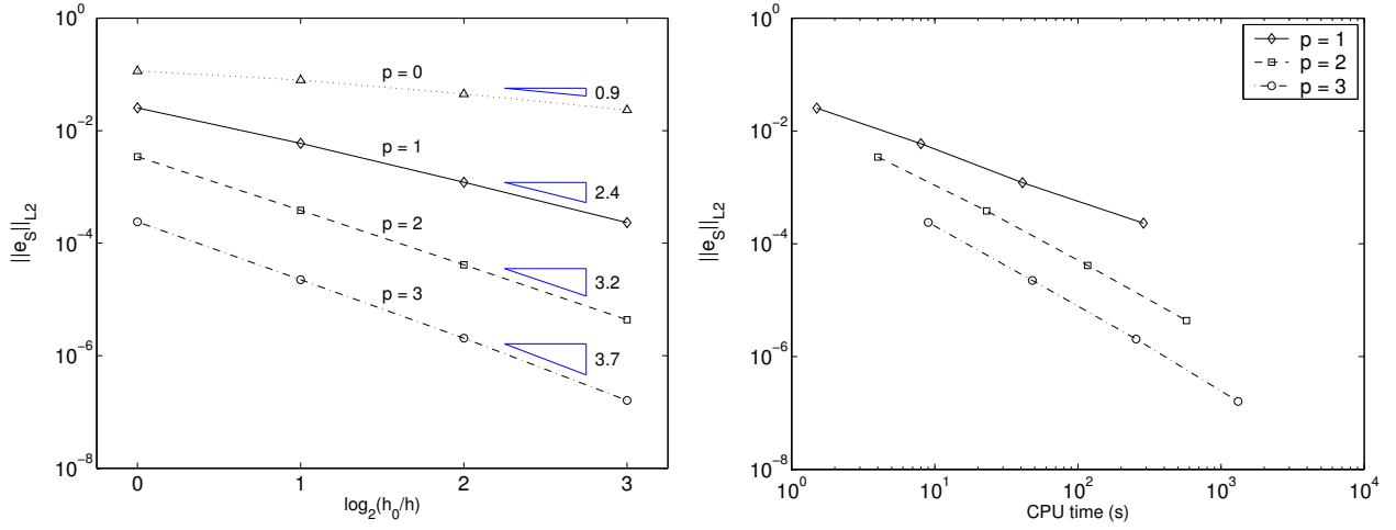
(a) Error vs. grid spacing
