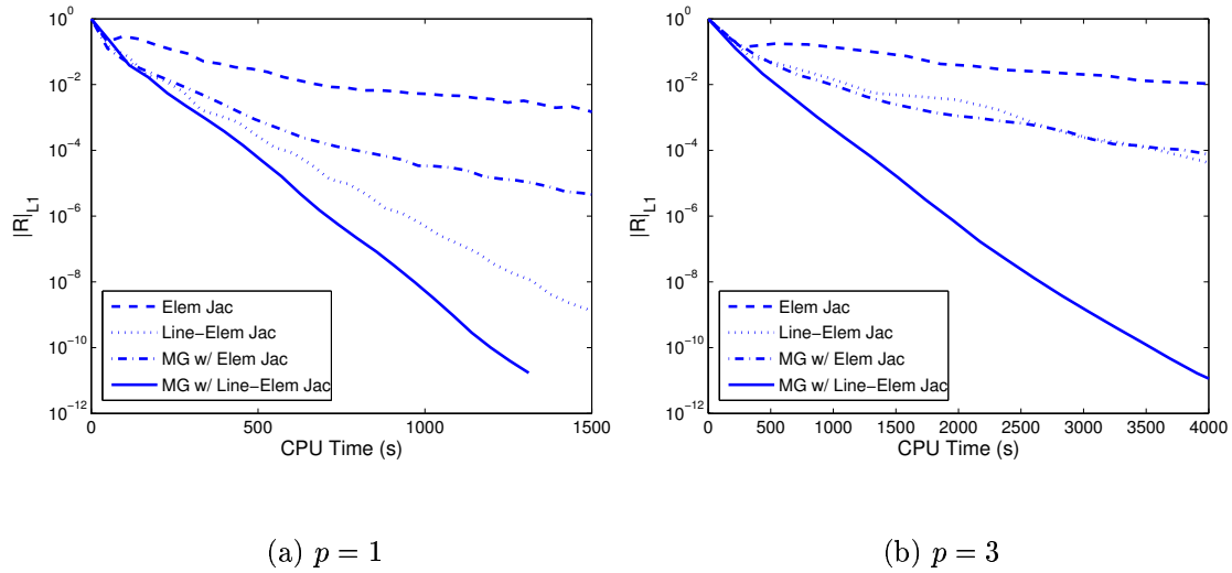
Figure 15: Solver comparison on 2688 element mesh for NACA 0012 at M = 0.5 , Re = 5000 , \alpha = 0^\circ .
