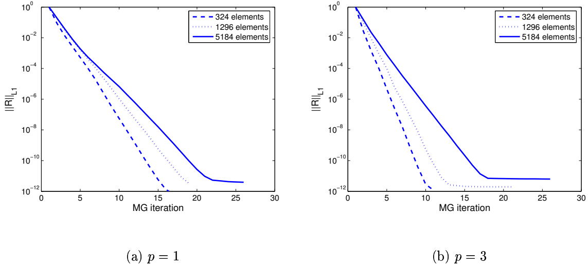
Figure 7: p -Multigrid residual convergence versus grid size, for inviscid duct flow at M = 0.5 .
