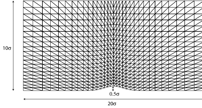
Figure 4: 1296 element mesh for flow over a Gaussian bump.
