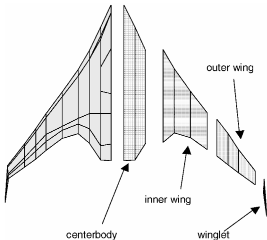
Fig. 3 Modular structural breakdown of BWB.
