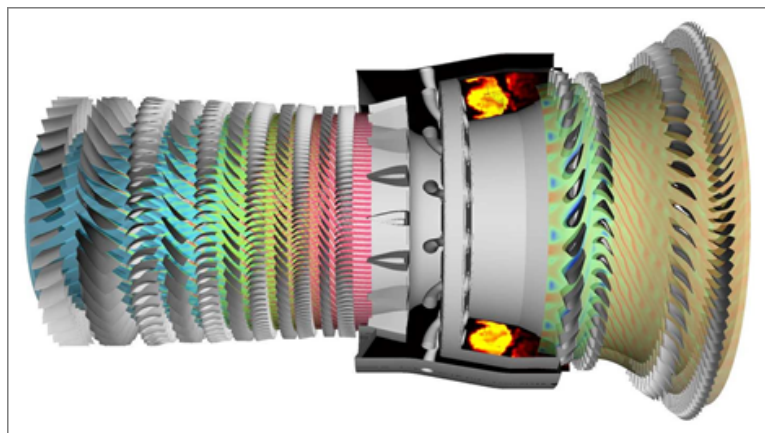
Figure 8. Simulation of 20-degree sector of the full high-spool of a Pratt & Whitney engine. Compressor and turbine shows axial momentum; combustor shows temperature. 37
