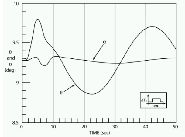
(b) Response to a step function throttle change of 0.1, from reference. 33
