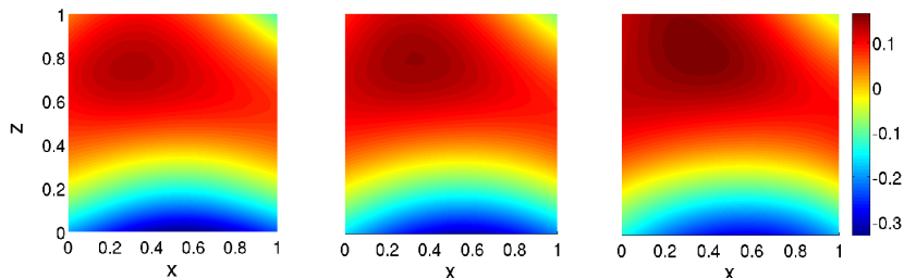
FIG. 5.8. The results of the MCMC solution to the 2-D N = N_p = 494 test case with reduction to n = n_p = 10 . On the left and right, respectively, we plot the lower and upper bounds of the \pm 2\sigma credible interval. The mean is shown in the center. Actual parameter field shown in Figure 5.5 (a). For reference, we show the projected actual parameter field below in Figure 5.5 (c). In comparison to the full MCMC solution, these results have a relative L_2(\Omega) error of 16.6%, 12.2%, and 16.3%, from left to right.
