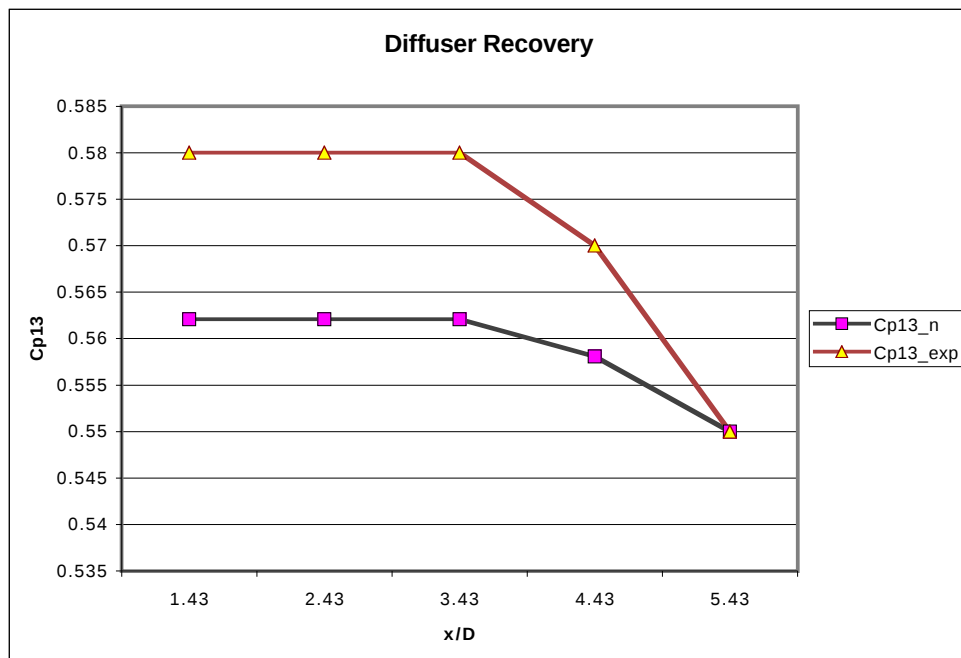
Figure 3-7: Overall Diffuser Static Pressure Recovery
