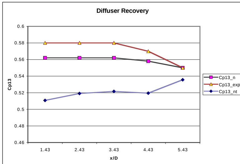
Figure 4-9: Overall Diffuser Static Pressure Recovery ( C_\tau = 10^3 )
