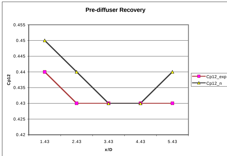
Figure 3-6: Pre-diffuser Static Pressure Recovery
