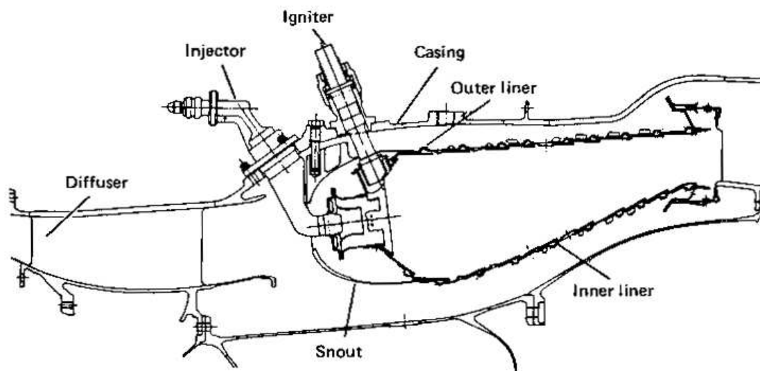
CF6-50 annular combustor (courtesy General Electric Company).
