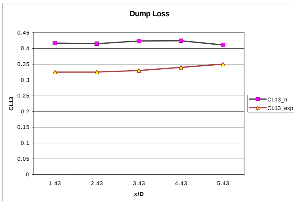
Figure 3-8: Overall Total Pressure Loss
