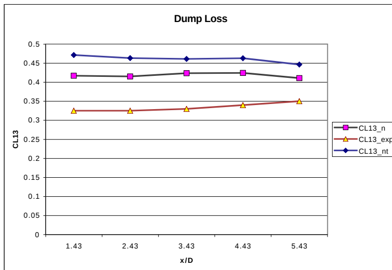
Figure 4-10: Overall Total Pressure Loss ( C_\tau = 10^3 )
