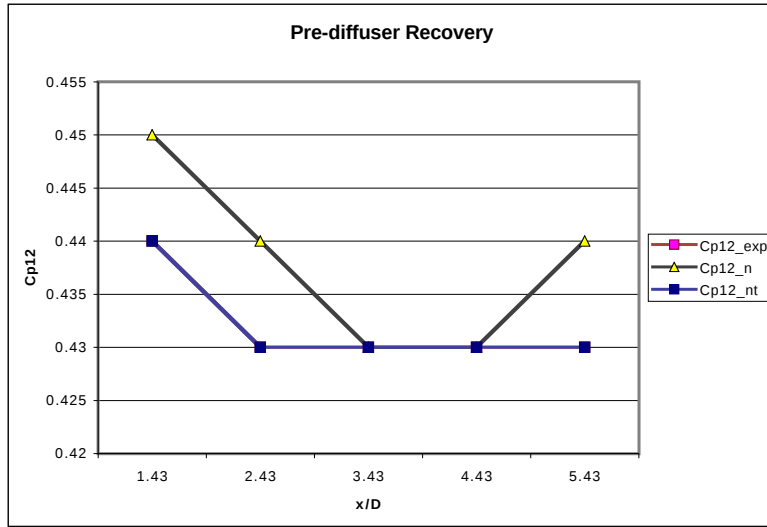
Figure 4-8: Pre-diffuser Static Pressure Recovery ( C_\tau = 10^3 )
