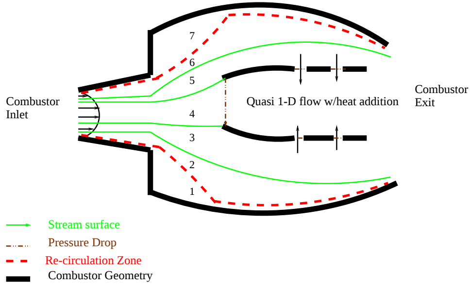
Figure 2-3: Combustor features
