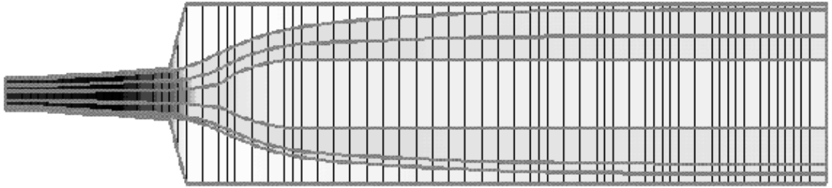
Figure 4-5: Flow Plot: Mach number ( C_\tau = 10^3 )
