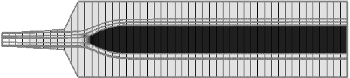
Figure 4-3: Flow Plot: Static Pressure Recovery
