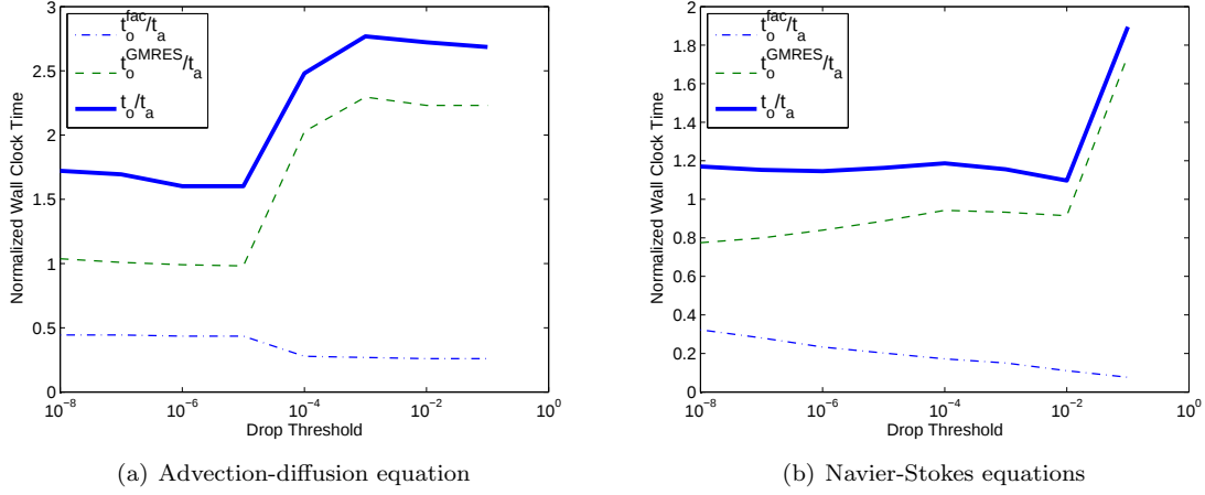
Fig. 16. Wall clock time for linear solver using ILUT on obtuse mesh normalized by the linear solver time using ILU(0) on acute mesh of 500 elements at R = 10^4
