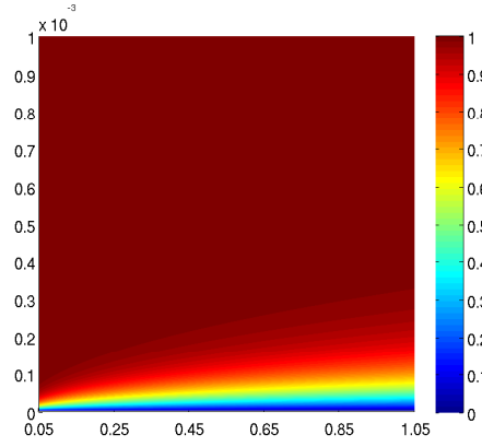
Fig. 1. Exact solution of u given in Eq. (6)
