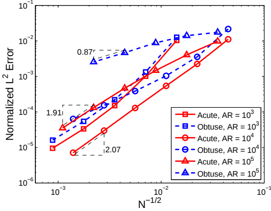
(a) Solution Order of k = 1
