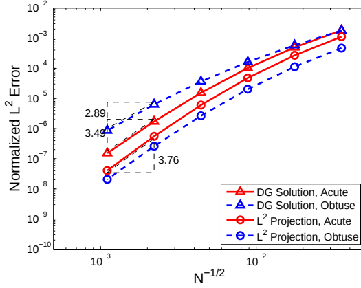
(b) Solution Order of k = 3
