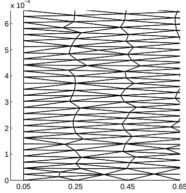
Fig. 11. Unstructured meshe
