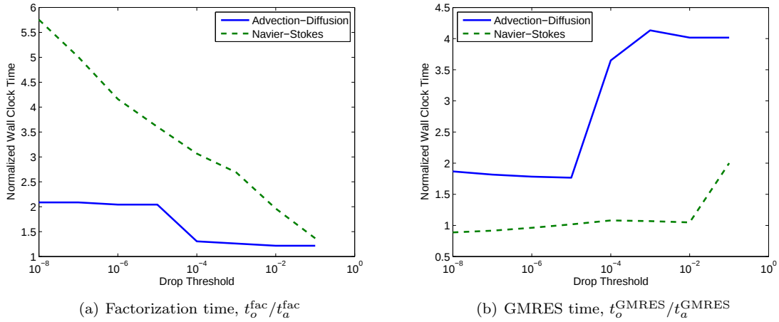
Fig. 17. Factorization time and GMRES time using ILUT on obtuse mesh normalized by the corresponding time using ILU(0) on acute mesh of 500 elements at R = 10^4
