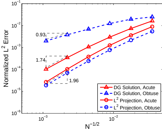
(a) Solution Order of k = 1
