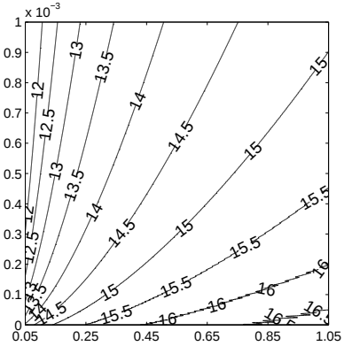
Fig. 3. \log_{10}(u_{\mathbf{e}_1}^{(4)}/u_{\mathbf{e}_2}^{(4)}) of u in Eq. (6)
