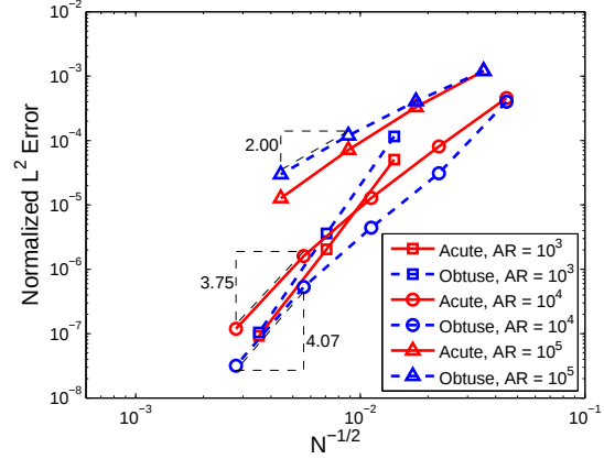
(b) Solution Order of k = 3
